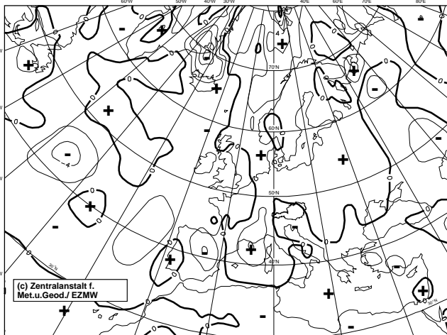
TEMP_adv510 [ 000/2 K/12H ] (DO,23.07. ) DO,23.07.2009 00 UTC
