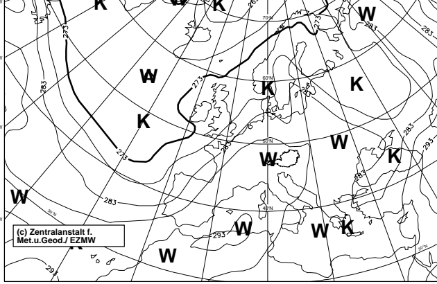
aeqRTP-T58 [ 273/5 K ] (DO,23.07. ) DO,23.07.2009 00 UTC
